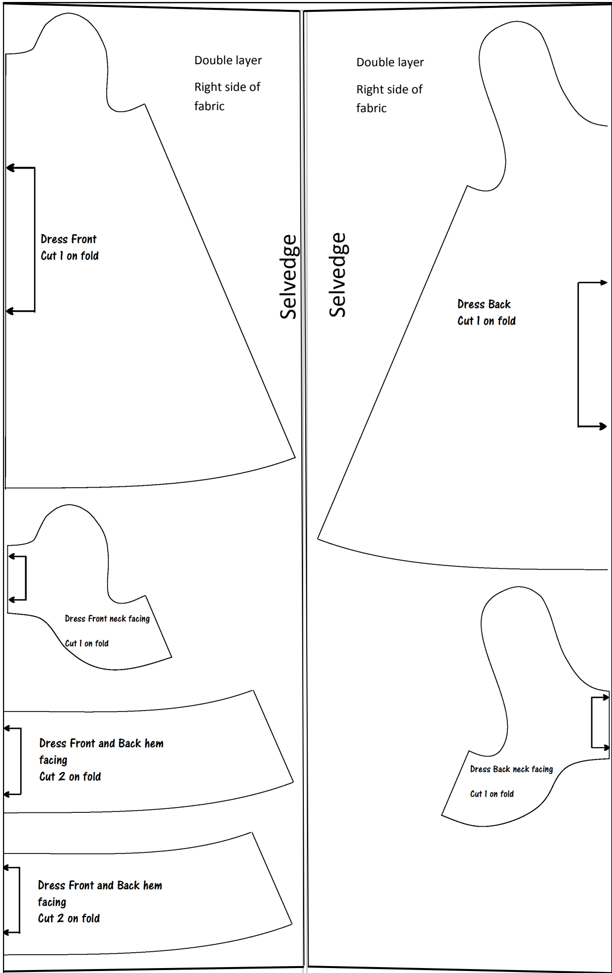
Layout for 150 cm wide fabric - fold so that selvedge meet in the centre
